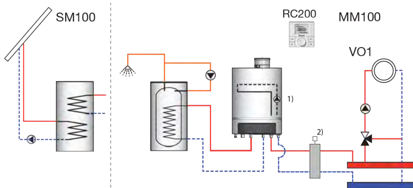
Logamatic RC200
